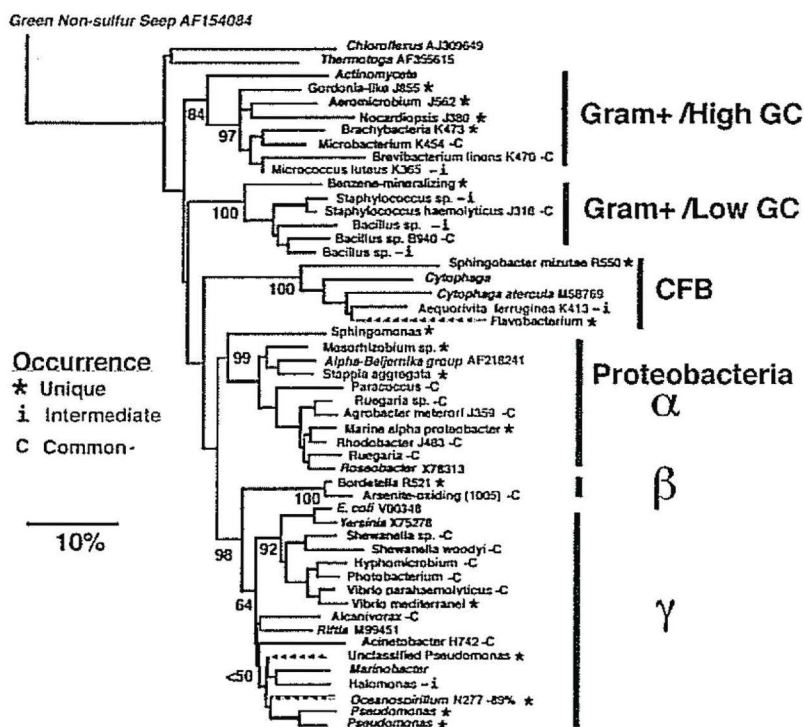
Fig. 3. Neighbor-joining phylogram based on 16S rRNA gene sequences of representative bacterial isolates. The tree was built with the PAUP 4* program (SWOFFORD, 1999) after deleting unalignable gapped regions, and bootstrap testing (with percentages shown at nodes). Isolates with sequences < 94 % similar to the closest GenBank BLAST match are shown with dotted lines.
