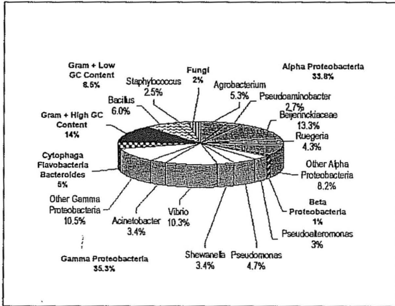
Fig. 2. The taxonomic distribution of the ~1000 isolates inventoried by RFLP to date as inferred by the RsaI and HaeIII RFLP patterns. Isolates were grouped based on these patterns, and representative 16S or 18S PCR products were sequenced from each group.
