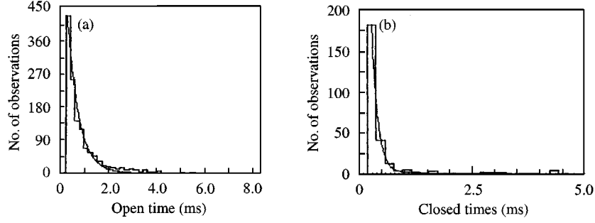
FIG. 2. Dwell time distributions to +40 mV for the channel shown in Fig. 1. (a) represents the open time and (b) the closed time distribution. The lines represent best fits of exponential functions to the experimental data points, using the Levenberg Marquardt algorithm. Number of events is 2330. Note that the histogram for the closed times has the abscissa expanded in order to better visualize the fitting. The exponentials are described in the text.
