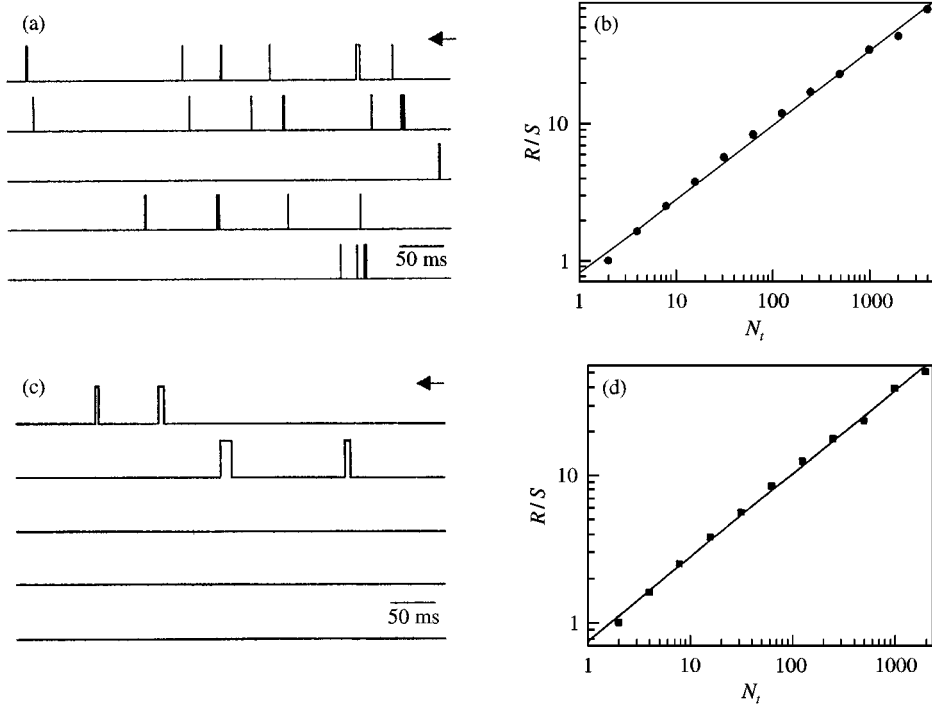
FIG. 3. R/S analysis applied to simulated single-channel data. The left panels (a) and (c) show three- and four-state Markovian models. Both simulations were done assuming the rate constants described in the text, at +40 mV. The right panels show double-logarithmic plots of R/S vs. N_t (size of the sample) for a typical simulation of the three [(b); H = 0.534 ; R = 0.998 ] and four-state [(d); H = 0.557 ; R = 0.997 ] Markovian models. Arrows indicate the open state of the channel. The continuous lines are best linear fits to the points and R is the correlation coefficient in each case.
