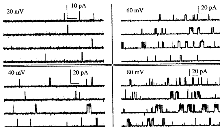
FIG. 1. Single-channel records of the calcium-activated potassium channel. The currents were recorded at the indicated voltages in the inside-out configuration. The solution of both pipette and bath were 150 mM KCl and the free calcium concentration was 10^{-7} M. Horizontal calibration bars indicate 50 ms.
