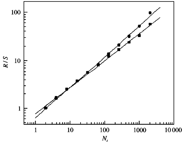
FIG. 4. R/S analysis for the channel shown in Fig. 1. R/S was calculated according to the text and plotted against N_r , the size of the sample. Data refer to the single-channel record observed at +40 mV before (●; H = 0.64 ; R = 0.998 ) and after randomly shuffling the experimental dwell times (■; H = 0.56 ; R = 0.998 ). R is the correlation coefficient.
