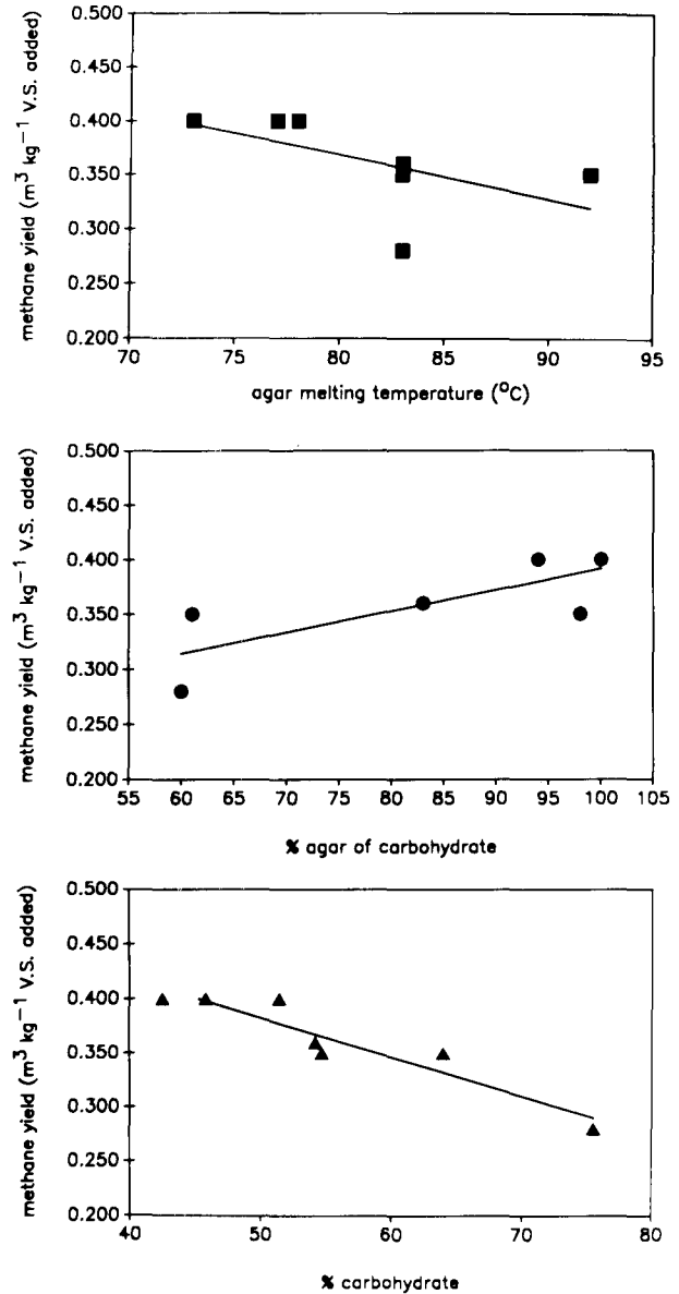
Fig. 1. Methane yield as a function of agar melting temperature (top), % agar of carbohydrate (middle), and % carbohydrate (bottom). The regression coefficients are r = 0.57 , 0.79 and 0.94 , respectively.
